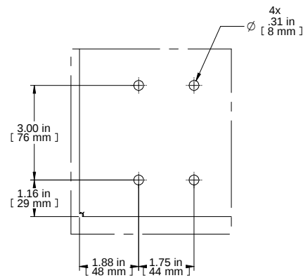
DETAIL A TYPICAL EACH CORNER
