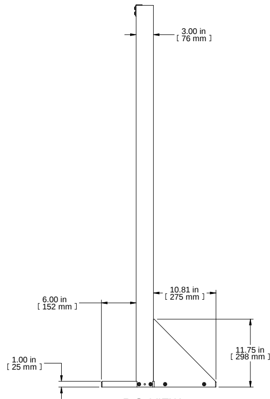
R.S. VIEW
